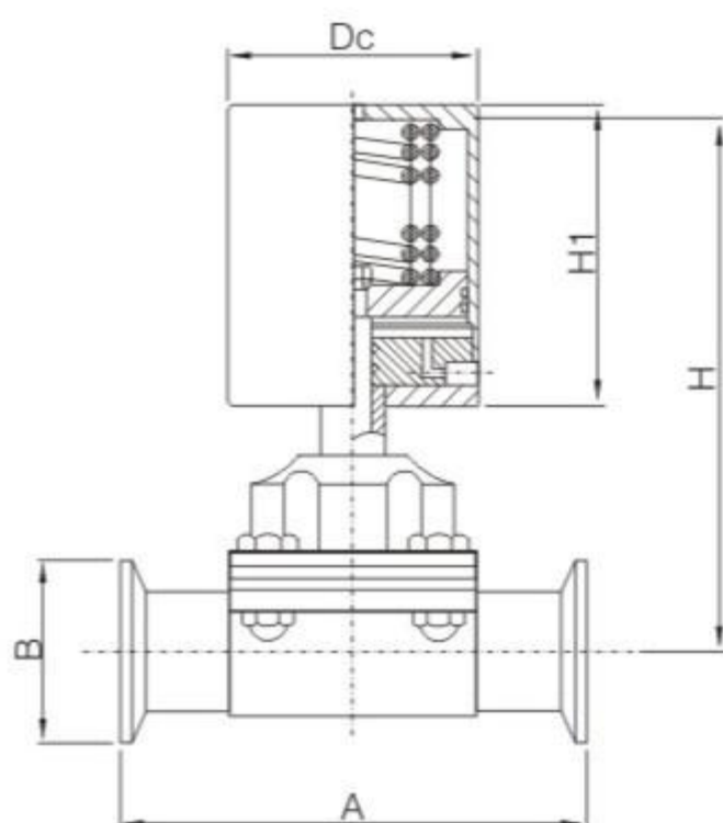
气动隔膜阀 3A Pneumatic Diaphragm Valve
