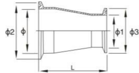
(同心Concentric)
