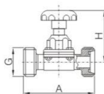
螺纹式隔膜阀 Threaded Diaphragm Valve DIN BUUD7013003
