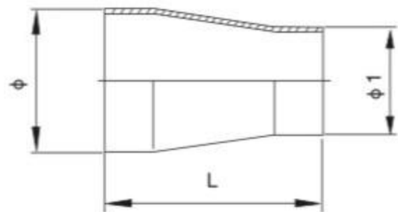
(同心Concentric)
